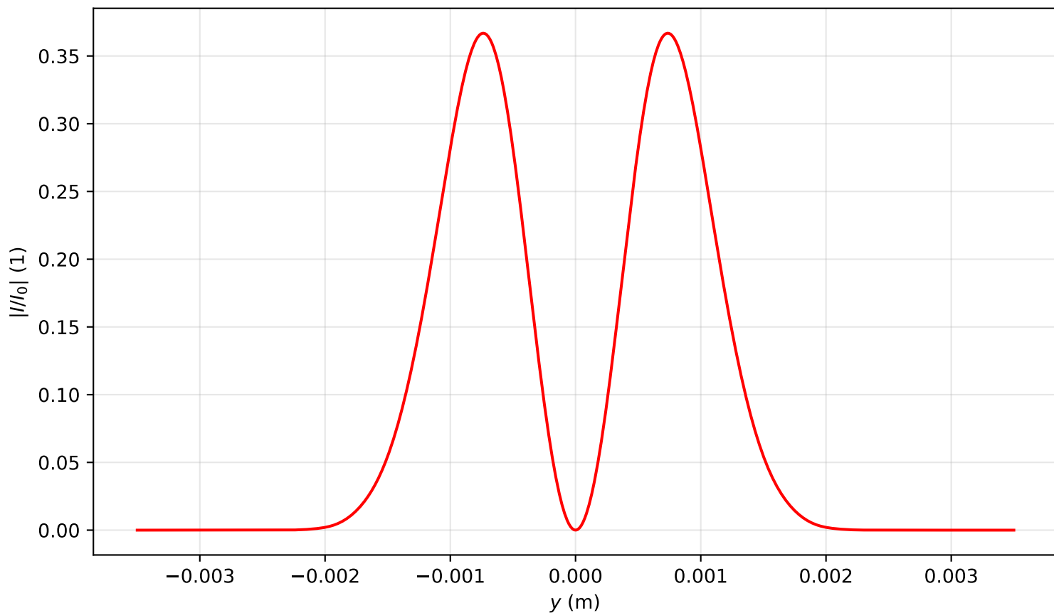
Intensity profile I(x=0, y, z=2.309)/I_0 , P_{in}=1.0P_{cr} , artificial time
